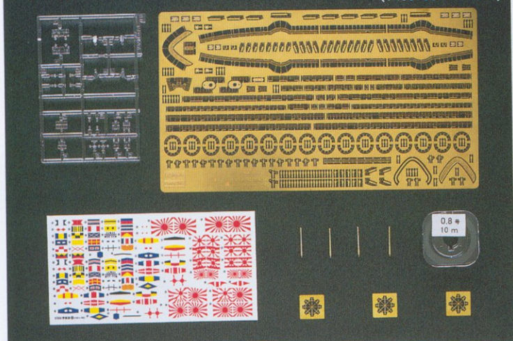
QG9 1:350 IJN DESTROYER TYPE KOH YUKIKAZE COMPLETION 1940 ETCHING PARTS (72109) (T4967834 72109 8)
